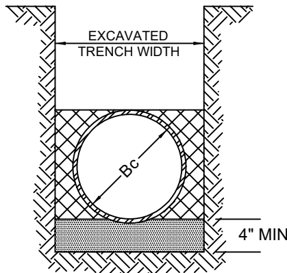
TYPE 4 PIPE BEDDED IN 4-INCH MIN. SAND, GRAVEL OR CRUSHED STONE; BACKFILL LIGHTLY CONSOLIDATED TO TOP OF PIPE
