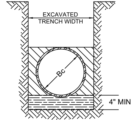
TYPE 3 PIPE BEDDED IN 4-INCH MIN. LOOSE SOIL; BACKFILL LIGHTLY CONSOLIDATED TO TOP OF PIPE
