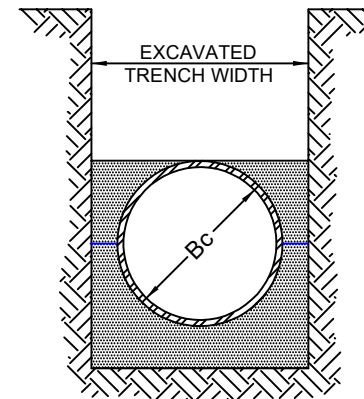
TYPE 5 PIPE BEDDED IN COMPACTED GRANULAR MATERIAL TO CENTERLINE OF PIPE; COMPACTED GRANULAR OR SELECT MATERIAL TO TOP OF PIPE
