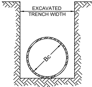
TYPE 1 FLAT-BOTTOM TRENCH; LOOSE BACKFILL
