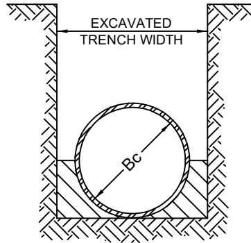
TYPE 2 FLAT-BOTTOM TRENCH; BACKFILL LIGHTLY CONSOLIDATED TO CENTERLINE OF PIPE
