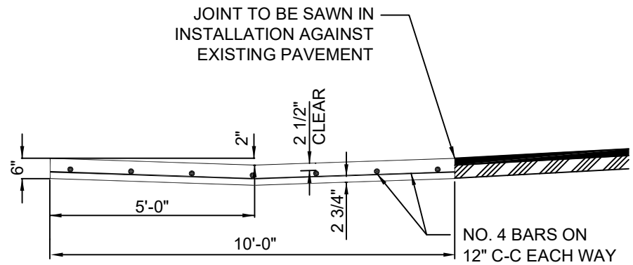
VALLEY GUTTER CROSS-SECTION
