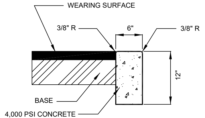
CONCRETE HEADER CROSS-SECTION
