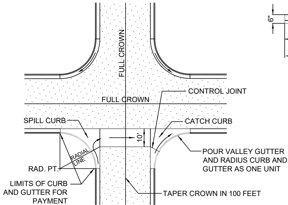
TYPICAL INTERSECTION WITH VALLEY GUTTER
